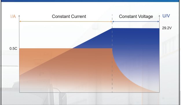
LiFePO4 Battery Charging Logic @0.5C
