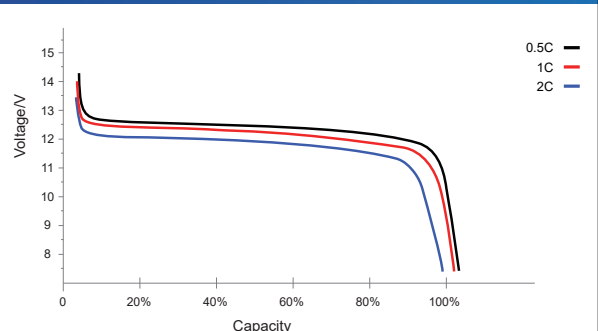
Discharge Characteristics At Various Rates
