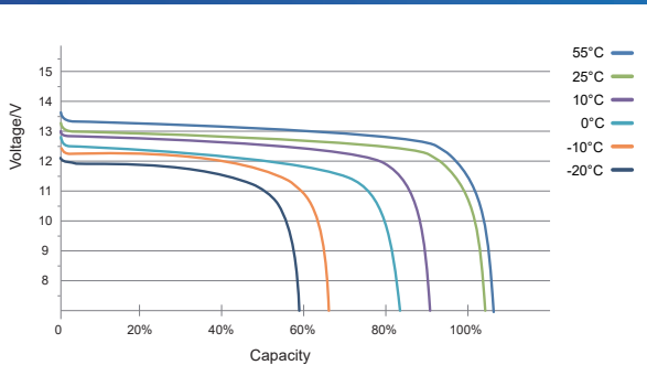
Discharge Characteristics At Various Temperatures
