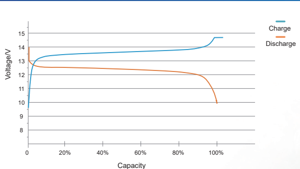
Charge & Discharge Voltage Characteristics
