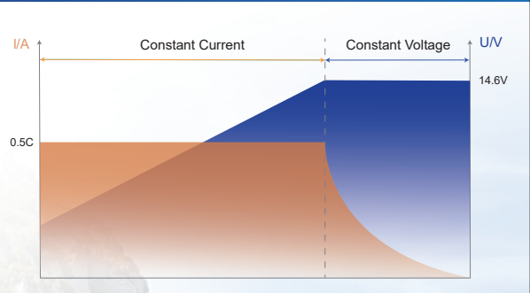
LiFePO4 Battery Charging Logic @0.5C
