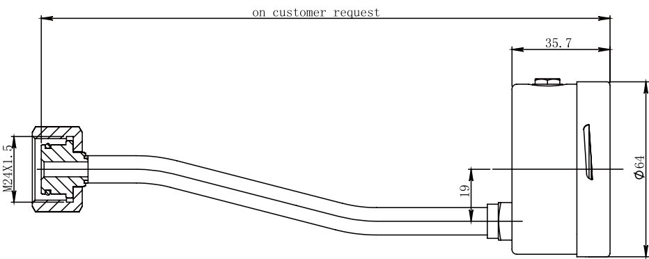
KL60 eccentric sample gauge size
