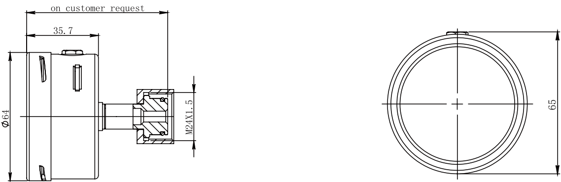
KL60 centerpiece sample gauge size
