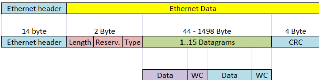
Fig. 22: Structure of an Ethernet frame with EtherCAT protocol data
