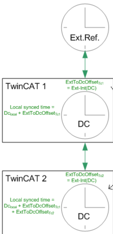
Fig. 298: Cascade consisting of controlled TwinCAT systems
