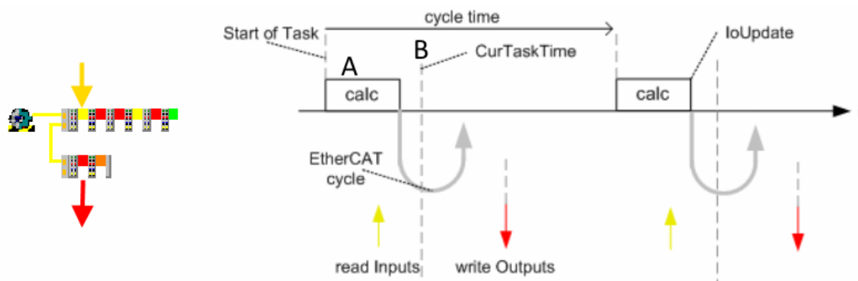
Fig. 267: Topology and principle of operation used in the example
