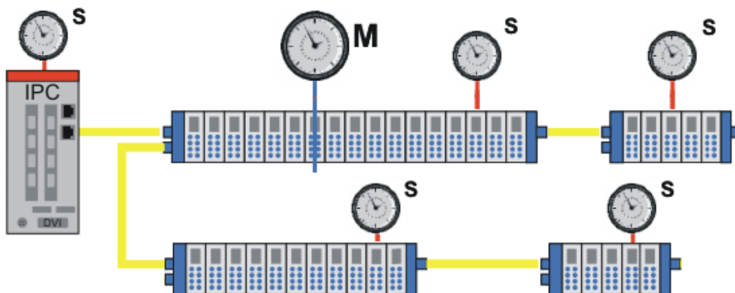
Fig. 212: topology of the EtherCAT system with DC-capable devices
