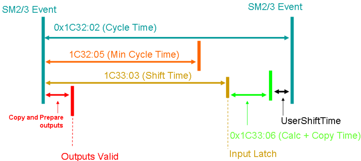
Fig. 288: Local cycle, synchronization with SM2/3 event, shifting of "Input Latch"
