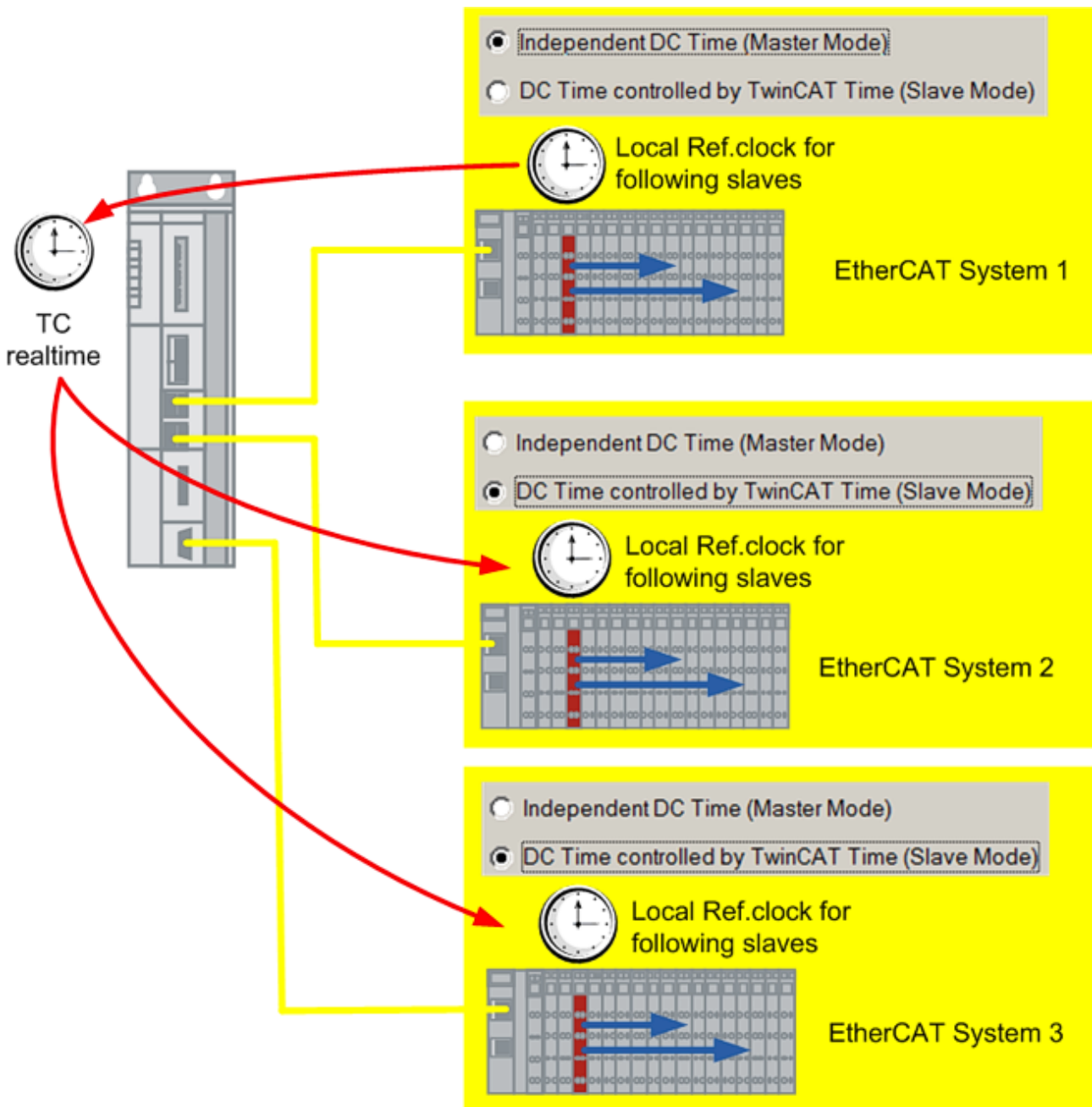
Fig. 228: DC-coupling of EtherCAT systems
