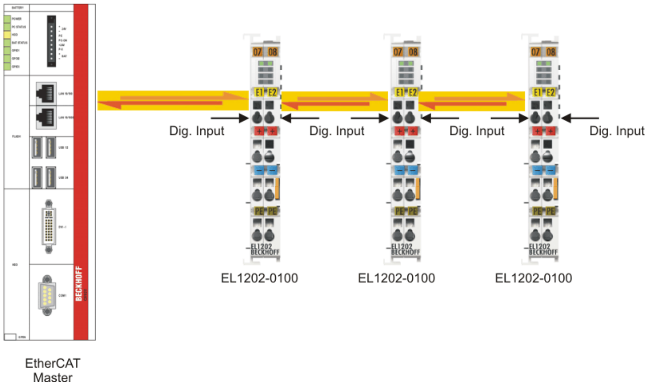
Fig. 258: Sample application with distributed clocks, cycle time 100 \mu s
