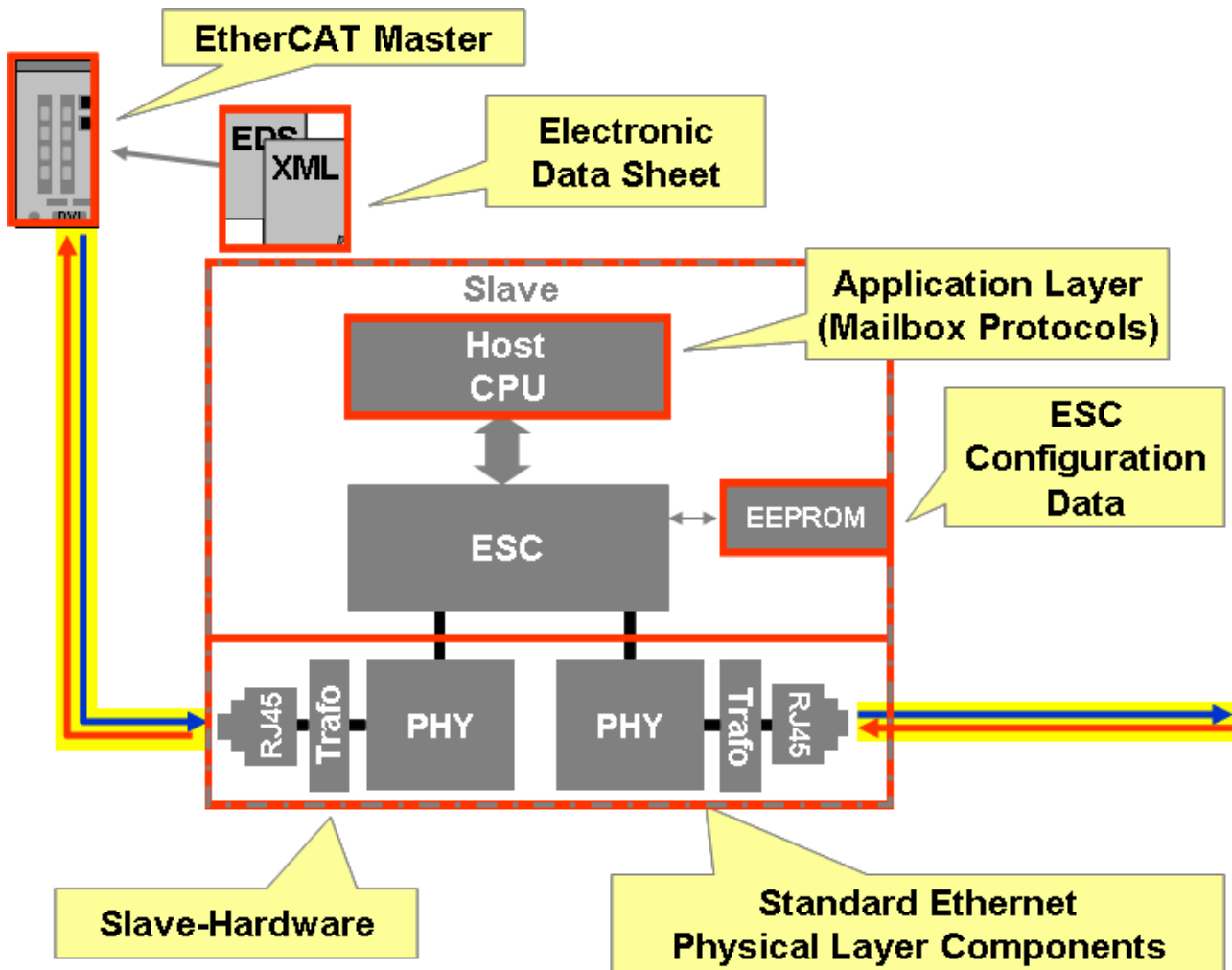
Fig. 255: Example for ESC functionality and embedding in a typical EtherCAT slave
