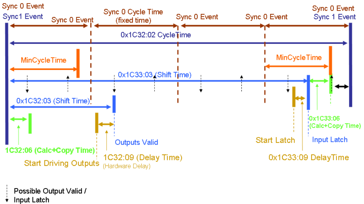
Fig. 291: DC, subordinate \mu C cycles, inputs/outputs delayed
