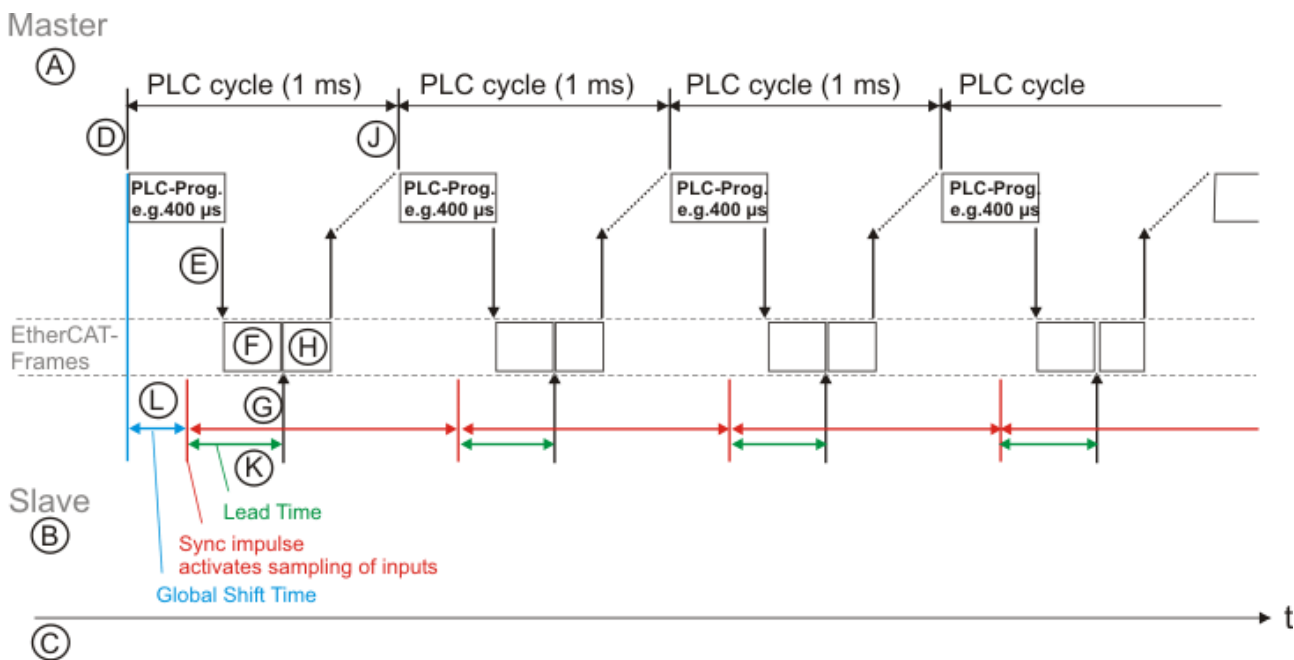
Fig. 259: EL1202-0100 read timing diagram
