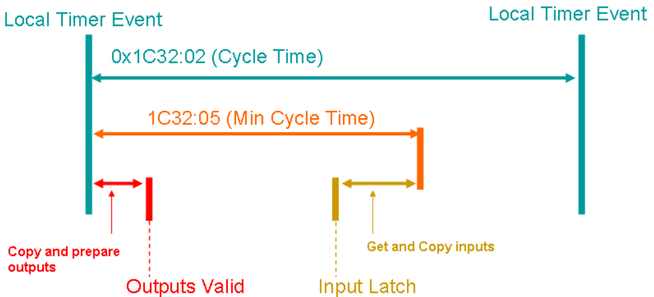
Fig. 286: Local cycle "Free Run" synchronization
