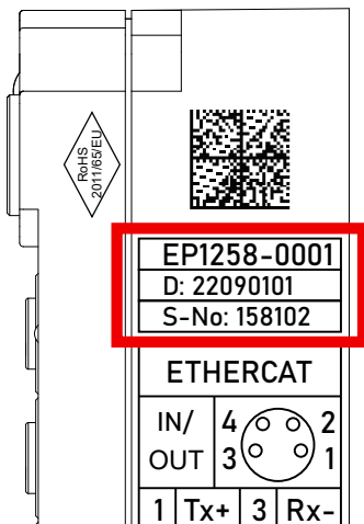
Fig. 142: EP1258-00001 IP67 EtherCAT Box with batch number/DateCode 22090101 and unique serial number 158102
