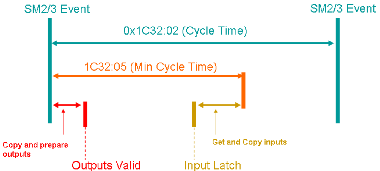
Fig. 287: Local cycle, synchronization with SM2/3 event
