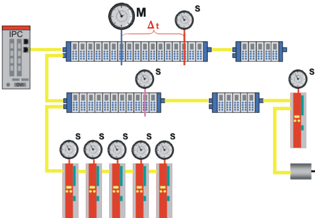
Fig. 256: Distributed clocks in the EtherCAT system
