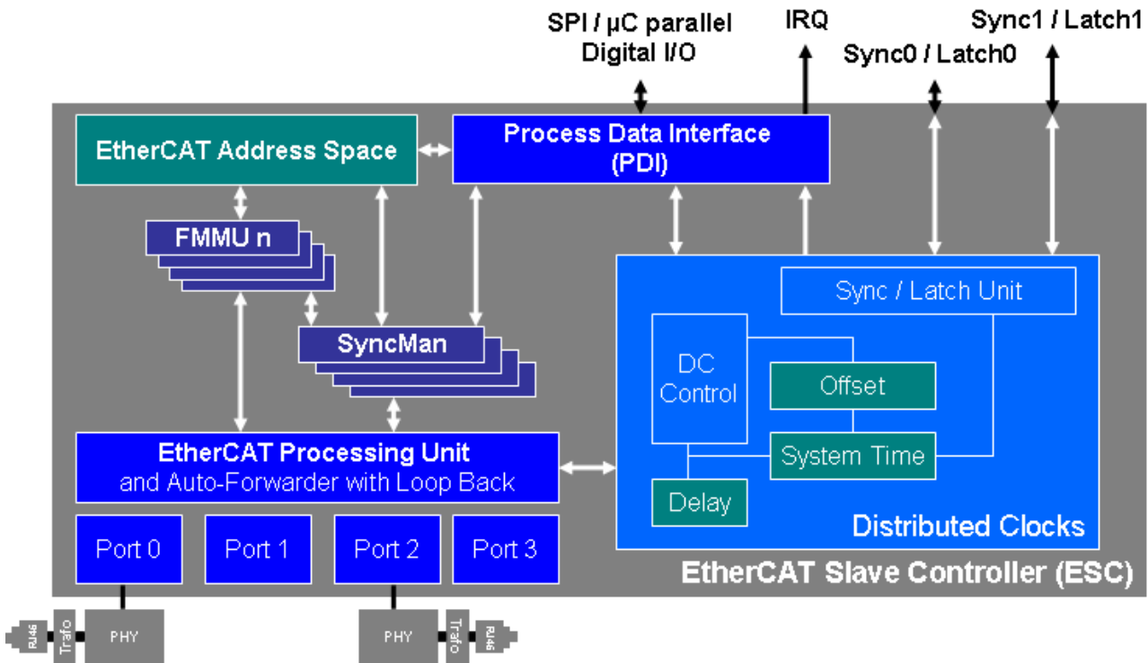
Fig. 257: Interfaces of the distributed clock unit
