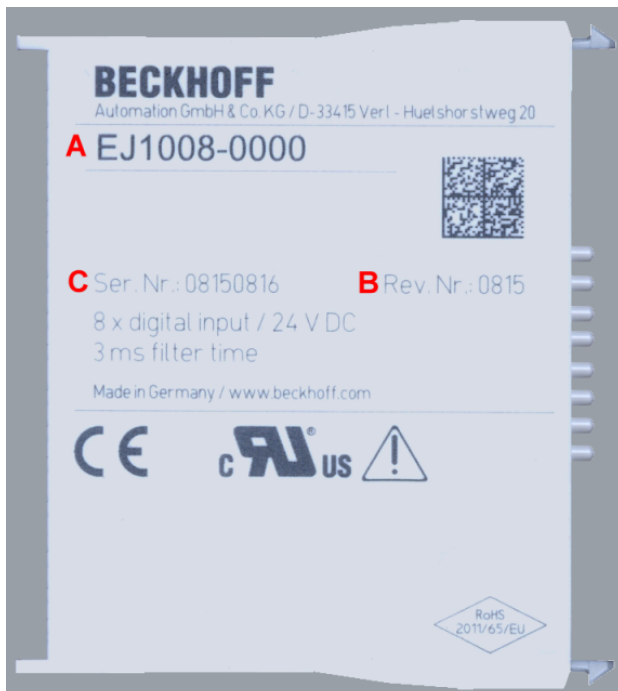
Fig. 140: Order identifier (A), Revision number (B) and serial number (C) using the example of EJ1008
