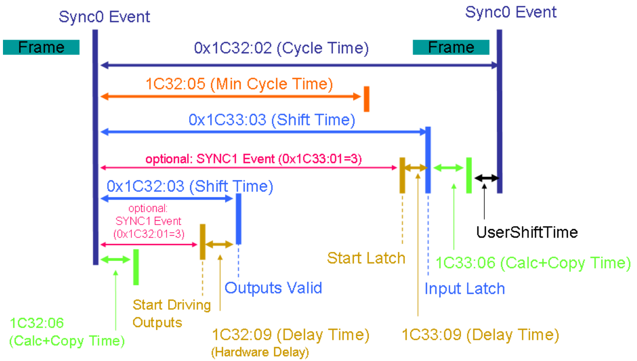
Fig. 290: Local cycle, synchronization with SYNC0 event, shifting of inputs/outputs
