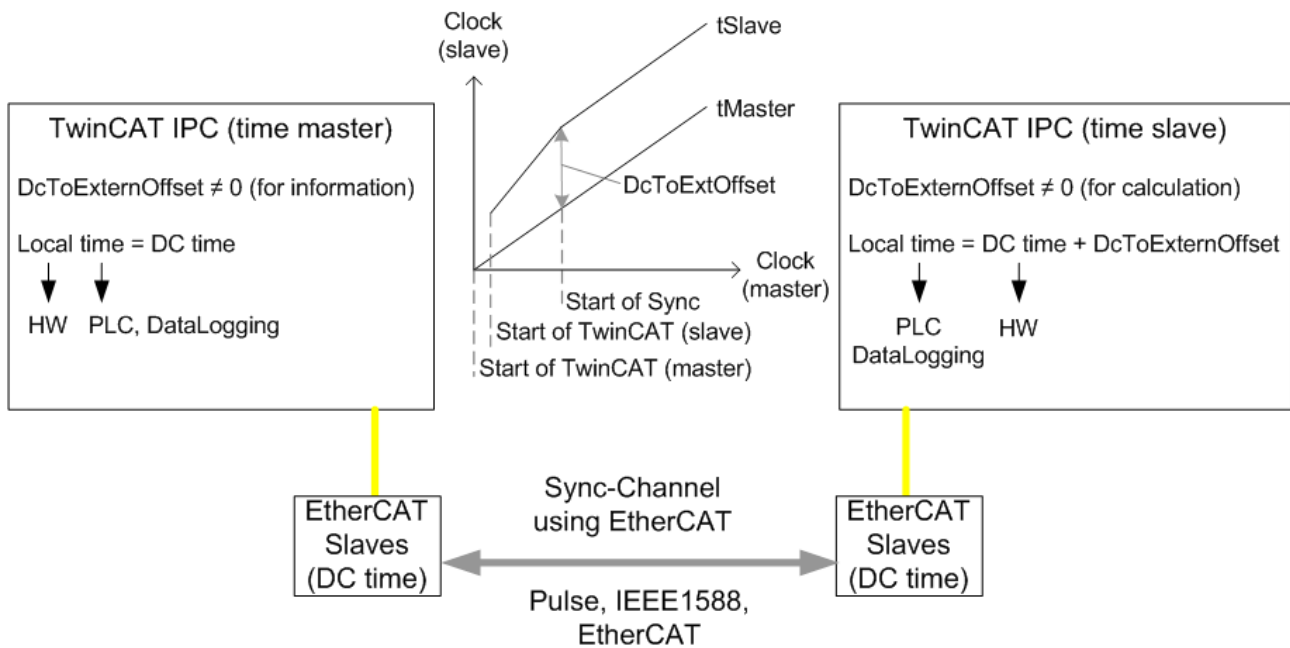
Fig. 297: Synchronization of 2 TwinCAT IPCs with the aid of EtherCAT components
