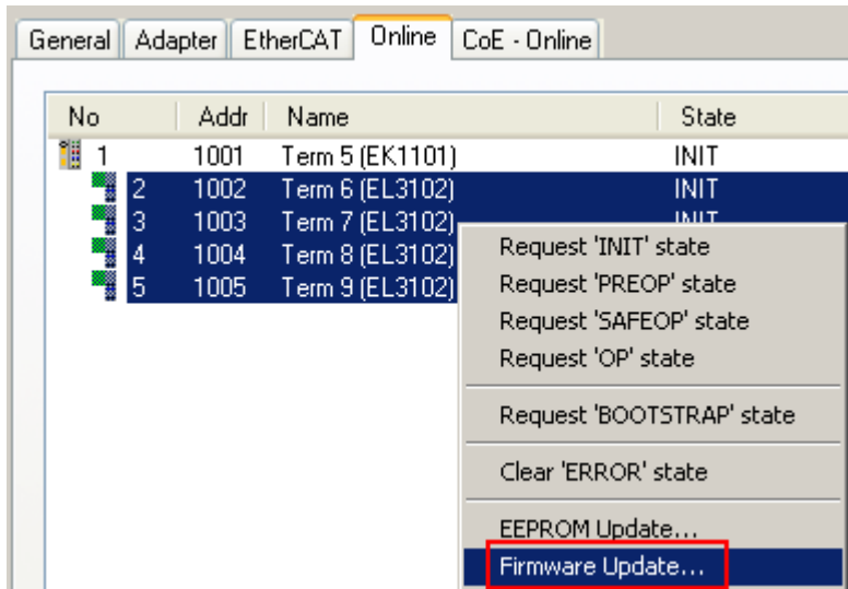
Fig. 345: Multiple selection and firmware update
