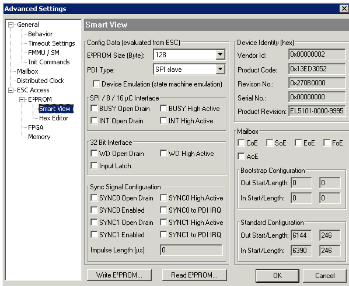
Fig. 332: Advanced Settings: "Smart View" dialog
