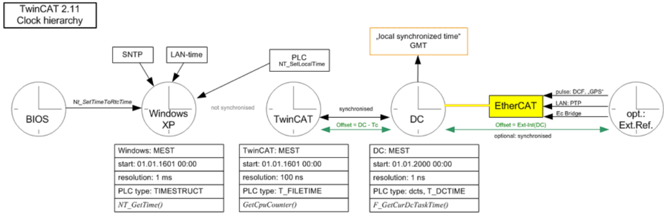
Fig. 295: TwinCAT 2.11 clock hierarchy (subject to change)
