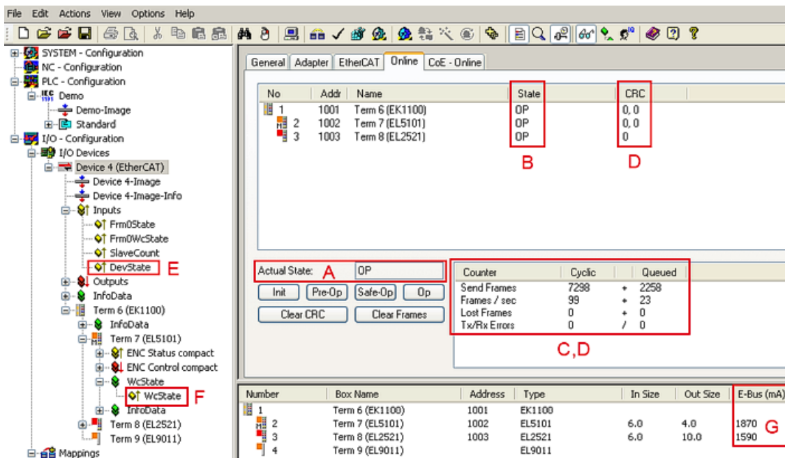
Fig. 202: online diagnostics for EtherCAT device
