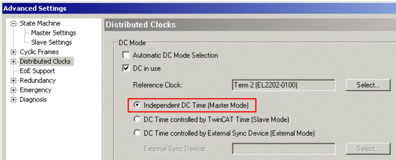
Fig. 305: Master PC works with its own ReferenceClock as a basis
