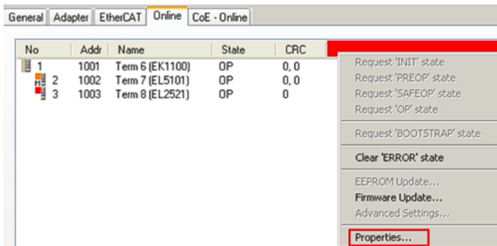
Fig. 223: display of additional register values from the slaves
