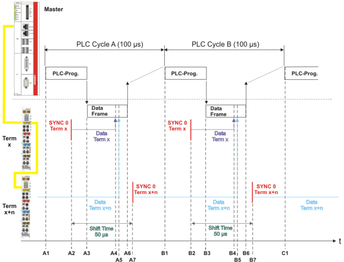
Fig. 266: Sample application for a manual shift time on SYNC0
