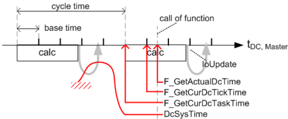
Fig. 285: Methods of reading the DC time
