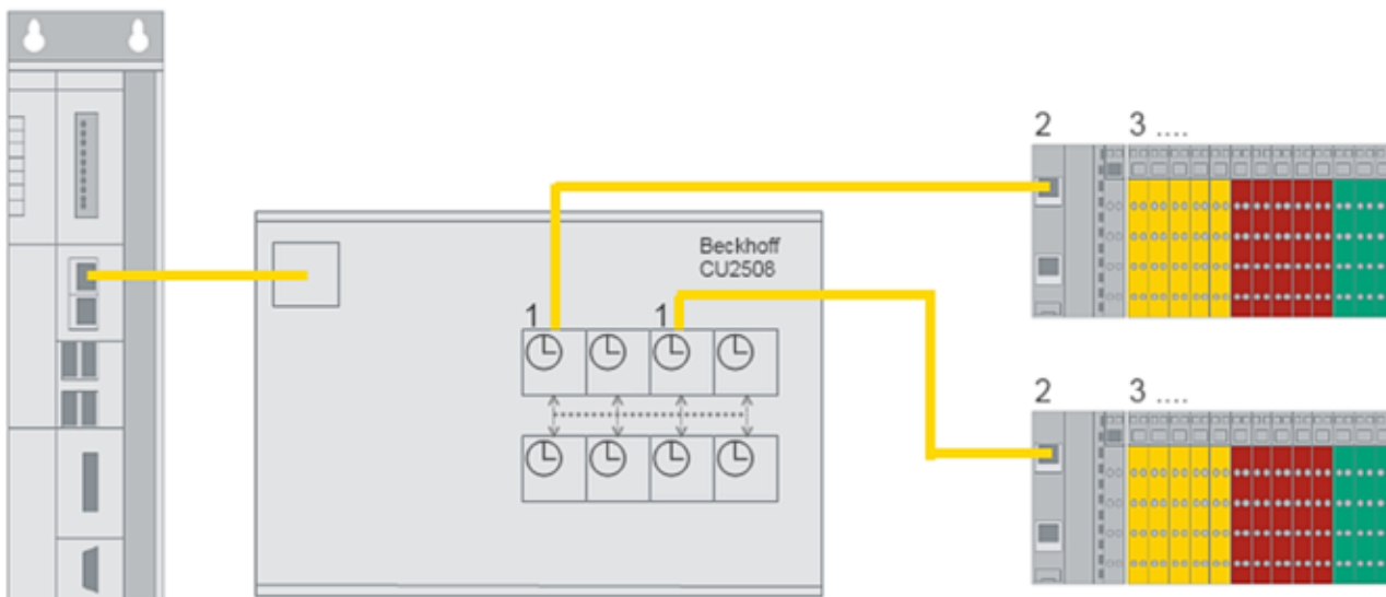
Fig. 229: EtherCAT topology with CU2508 and 2 EtherCAT systems
