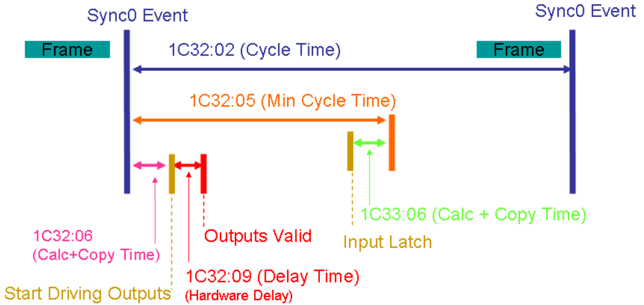
Fig. 289: Local cycle, synchronization with SYNC0 event
