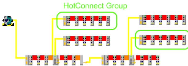
Fig. 30: Star topology
