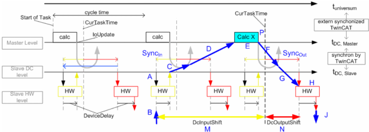
Fig. 270: EtherCAT Update (schematic)
