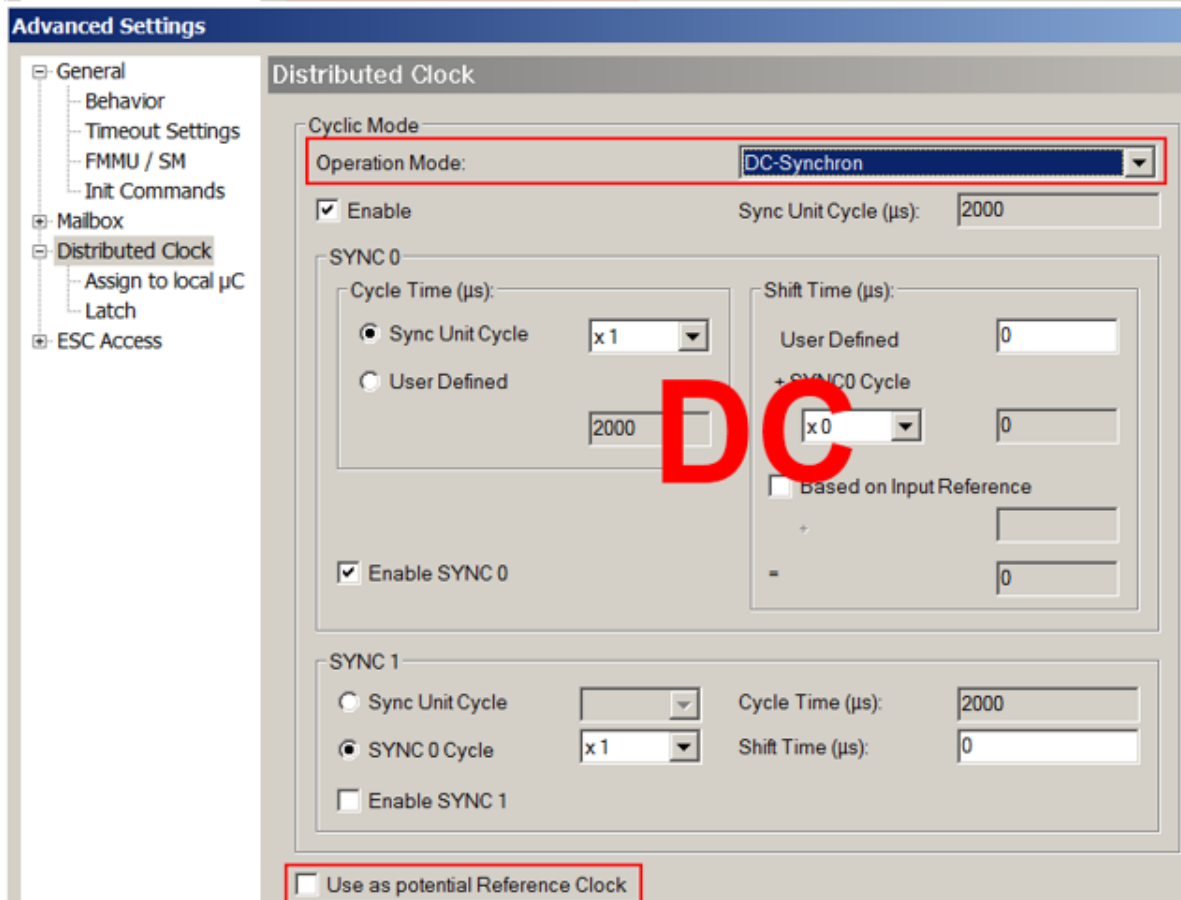
Fig. 221: Default slave setting – slave with and without DC capability
