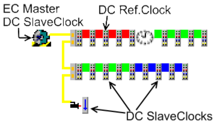
Fig. 249: mapping of DC to the topology
