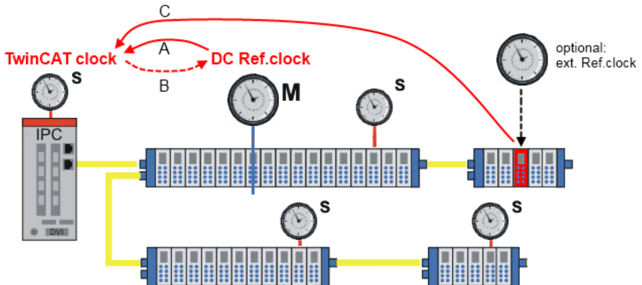
Fig. 226: distributed clocks system topology
