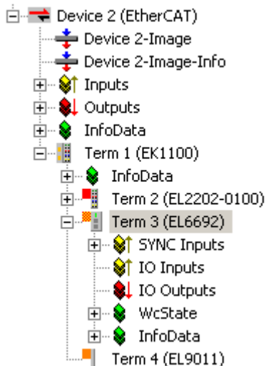
Fig. 300: Device on the master side
