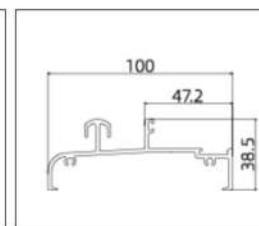
GH-TM21003 (Track)
