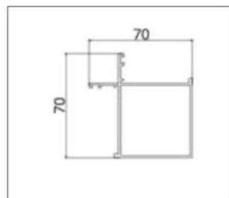
LB-PK5008(90° Corner)
