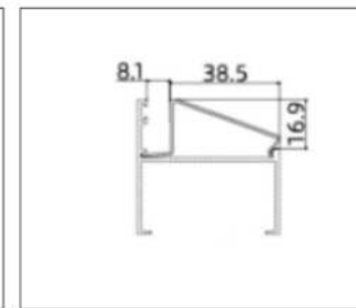
LB-PK5005(8.1)
