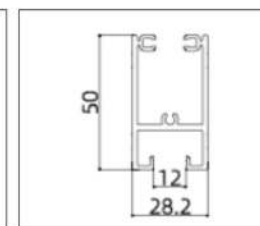
GH-TM21005 (Door Rail)
