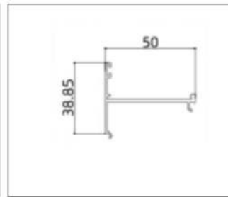
BG-PC50104 (Frame)
