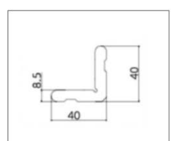
LB-PK5007 (Corner Connector)
