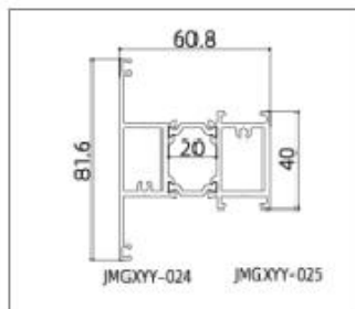
JMGXYY-GPM65102 (Mullion)
