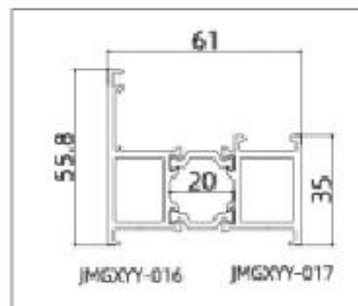
JMGXYY-GPM65101 (Frame)
