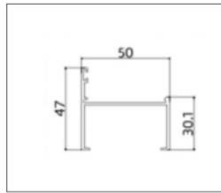
LB-PK5001-1.35 (Frame)
