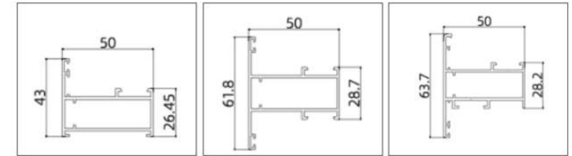
GZF5002 (Frame)
