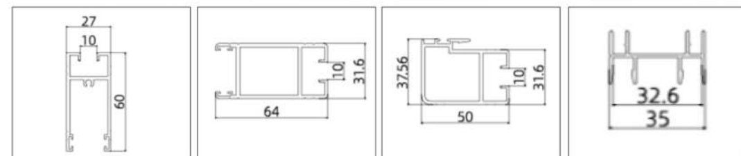
AL-9005-2.0 (Door Rail)
