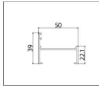
LB-PK5011-1.4 (Frame)
