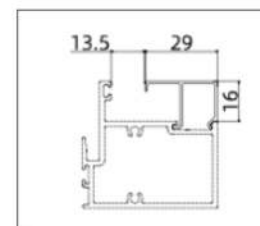
GH-TM21007 (Glazing Bead)
