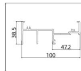
GH-TM21001 (Track)
