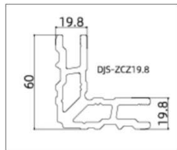
DJS-ZCZ19.8(Frame)
