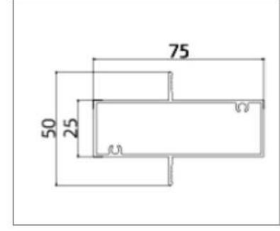
AB8006A (Transom)
