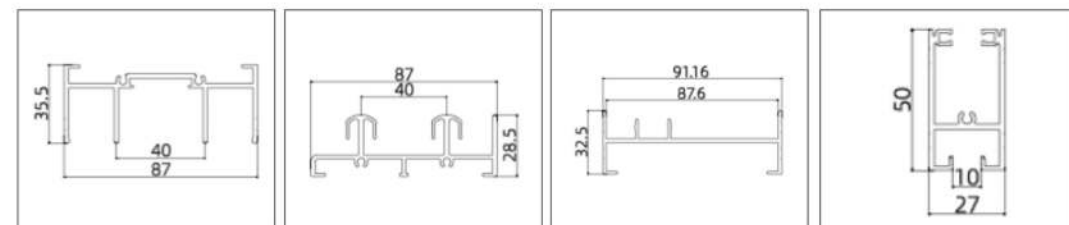
AL-9001-2.0 (Track)
