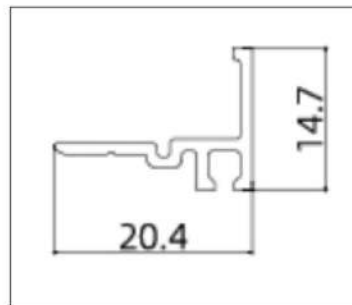
Jamb(Tooling Pending)
