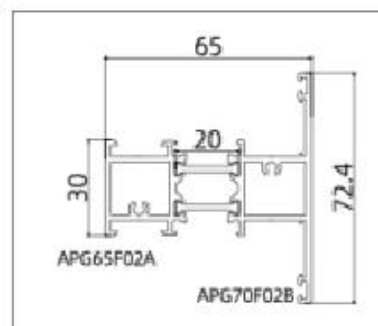
APG65F02 (Mullion)
