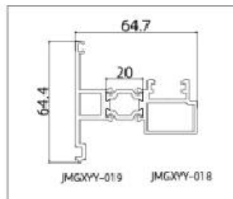
JMGXYY-GPM65106 (Mullion)
