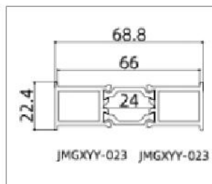
JMGXYY-GPC65108 (Mullion Bar)
