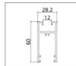
GH-TM21015 (Door Rail)
