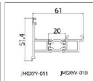
JMGXYY-GPM65104 (Frame)
