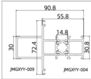
JMGXYY-GPC55102 (Mullion)
