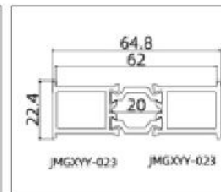
JMGXYY-GPM65108 (Mullion Bar)
