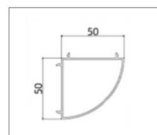
LB-PK5006(90° corner)
