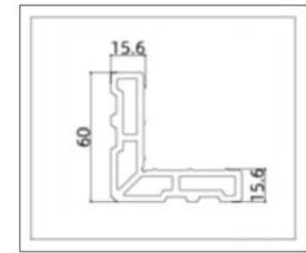
BG-PC50103 (Corner Connector)
