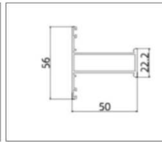
LB-PK5002-1.35 (Mullion)
