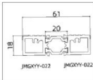
JMGXYY-GPM65107 (Bottom Rail)
