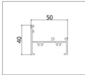
AL-PKC5002 (Mullion)
