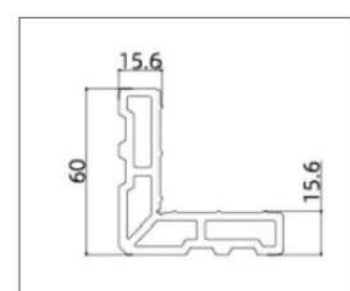
AL-PKC5013 (Corner Connector)
