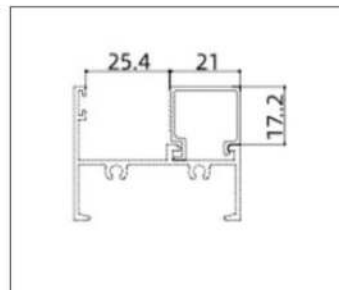
AL-PKC5005 (Glazing Bead 25.4)
