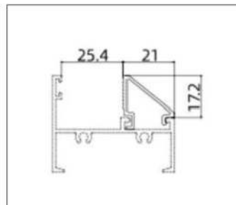
AL-PKC5007 (Glazing Bead 23)
