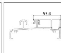
GH-TM21017 (Glazing Bead)
