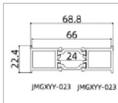
JMGXYY-GPC65108 (Mullion Bar )
