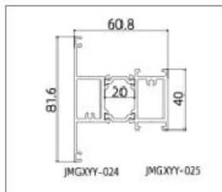
JMGXXY-GPM65102 (Mullion)
