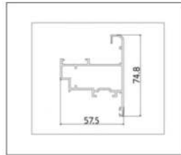
XD-5009NG (Vent)
