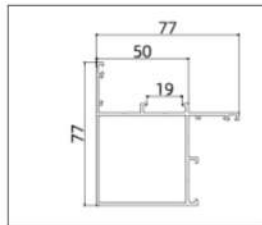
XD-5007ZND (90° Corner)
