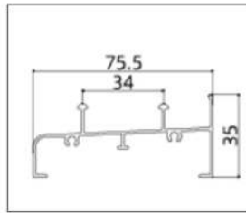
AB8002-0.95 (Track)
