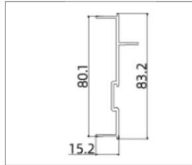
XLH-85TC002 (Frame Cover)
