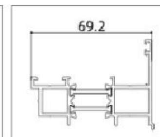
Adapter Profile (Mold Pending)
