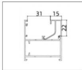
XD-5004G (Glazing Beadr)
