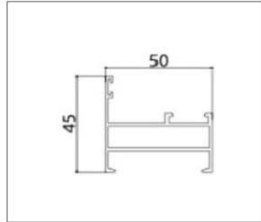
ALP7011 (Frame)
