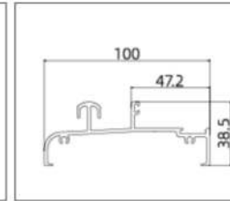
TC119002 (Track)
