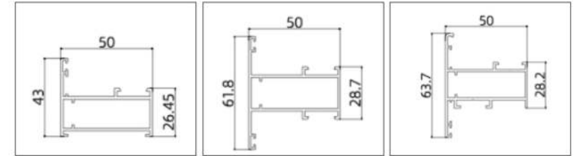
GZF5002 (Frame)
