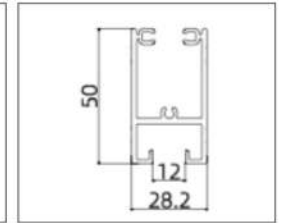
TC119006 (Lock Stile)
