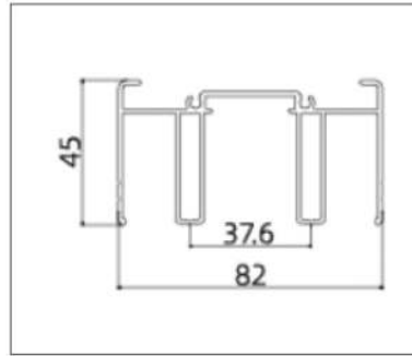
AK8201 (Top Track)
