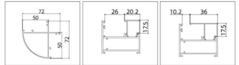
GZF7001 (90° Corner)
