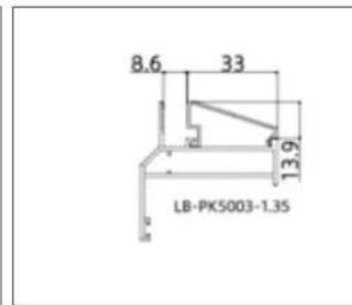
LB-PK5005 (Glazing Bead 8.6)
