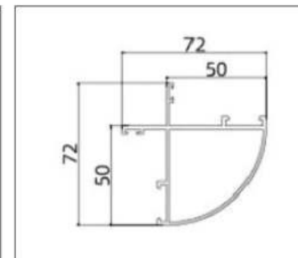
AL-PKC5009 (90° corner)
