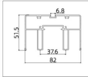
AK8201 (Roller Track)
