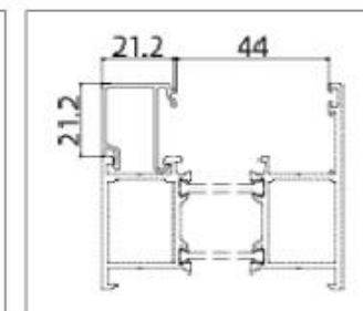
APG70F040 (Glazing Bead)
