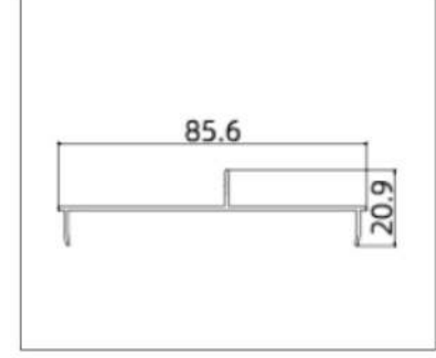
GH-85T08 (Frame Cover)
