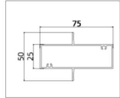
AB8006A (Transom)
