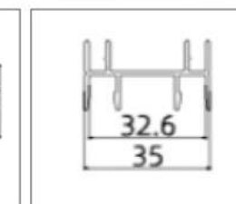
AL-9008-2.0 (End Cap)
