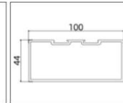
GH-GD001 (Mullion Bar)
