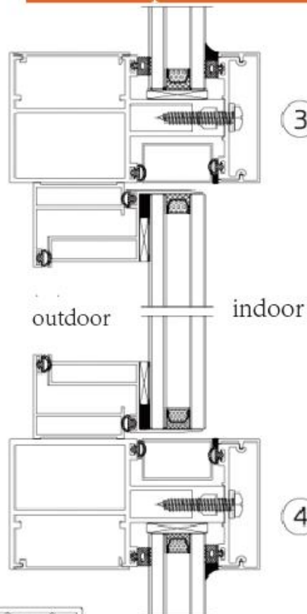
KQS13001(Mullion) Thickness:3.0mm Weight: 4.125kg/m KQS13002( ) Thickness:2.5mm Weight: 2.702kg/m KQS13003(reinforcing core) Thickness: 2.2mm Weight: 2.06kg/m YLH06BC(Frame Cover) Thickness:1.5mm Weight: 0.268kg/m
