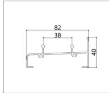
A8203 (Track)
