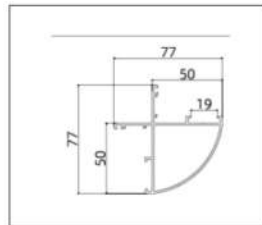
XD-5007 (90° Corner)
