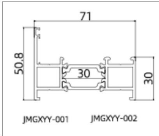
JMGXYY-GPC70101 (Frame)
