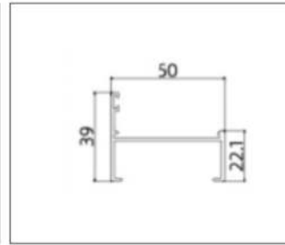
LB-PK5011-1.4 (Frame)
