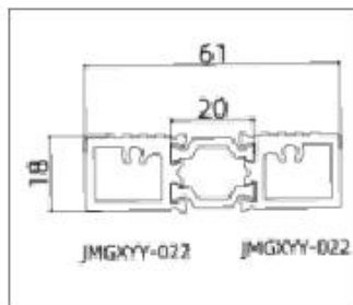
JMGXXY-GPM65107 (Bottom Rail)
