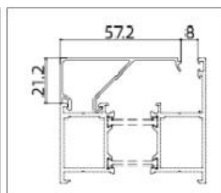
APG70F20 (Glazing Bead)
