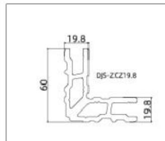
DJS-ZCZ19.8 (Guide Rail)
