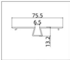
AB8009 ( Interlock)
