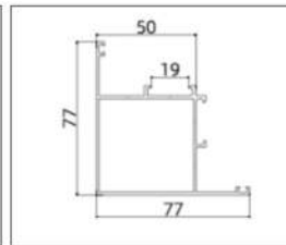
XD-50072N (90° Corner)
