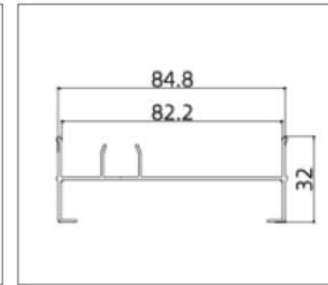
GH-85T03 (Frame)
