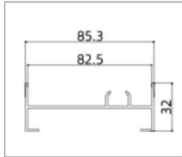
AK8203 (Frame)
