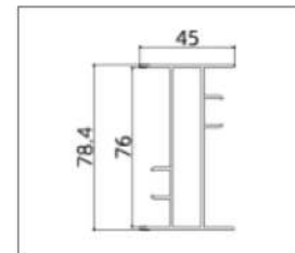
AB8024-1.2 (Double Jamb)
