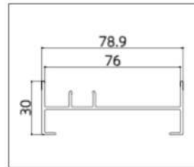
AB8004-1.35A (Frame)
