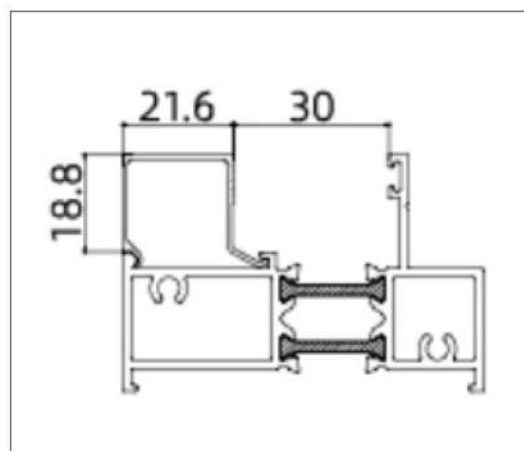
XLH-70PC005 (Glazing Bead)
