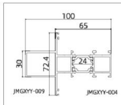
JMGXYY-GPC65102 (Mullion )
