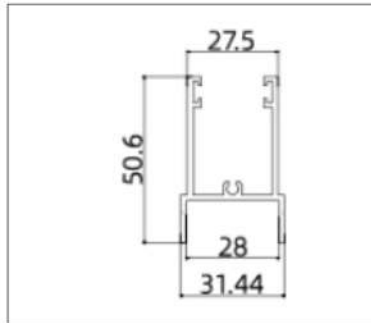
XLH-85TC007 (Door Rail)
