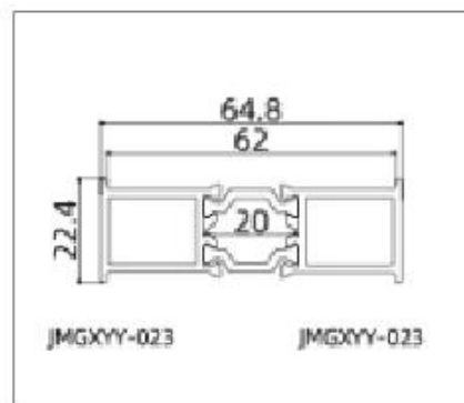
JMGXYY-GPC60108 (Mullion Bar)
