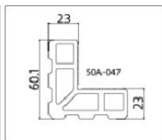
50A-047 (Corner Connector)
