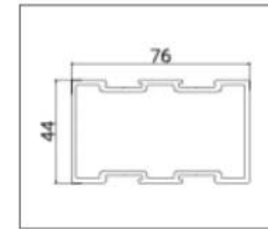
GH-GD003 (Mullion Bar)
