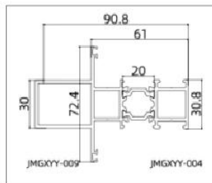
JMGXYY-GPC60102 (Mullion)
