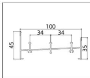
AB8016B ( Track)
