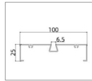
AB8018 (Frame)
