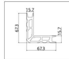
BFUS20922 (Corner Connector)
