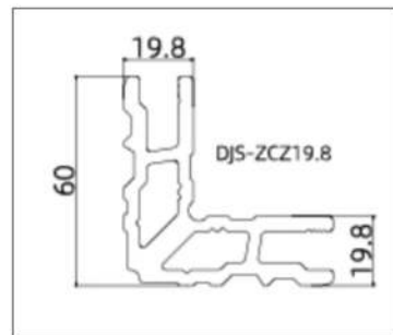
DJS-ZCZ19.8(Frame)
