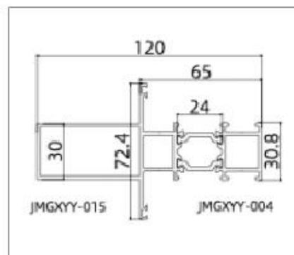
JMGXYY-GPC65112 (Mullion )
