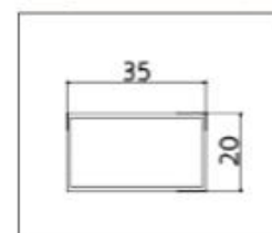
KQS15009(End Cap) Thickness: 1.0mm Weight: 0.288kg/m
