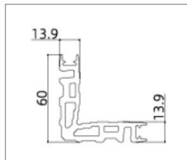
MD13.9A (Corner Connector)
