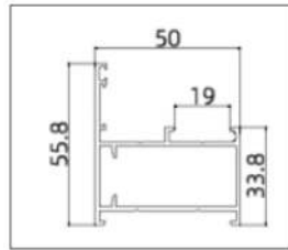
XD-5001G (Frame)
