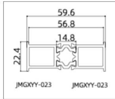
JMGXYY-GPC55108 (Mullion Bar)
