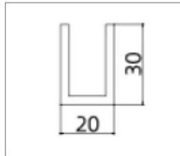
TZ-U3*20*30 (Mullion Connector)
