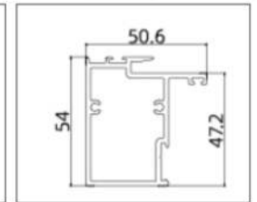
TC119020 (Frame Cover)
