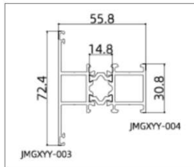
JMGXYY-GPC55122 (Mullion)
