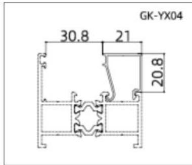
GK-YX04 (Glazing Bead)
