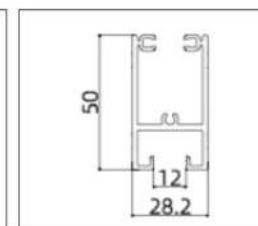
GH-TM21005 (Door Rail)
