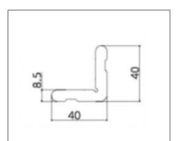
LB-PK5007 (Corner Connector)
