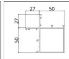
XD-507Z(90° Corner)
