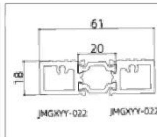
JMGXXY-GPM60107 (Bottom Rail)
