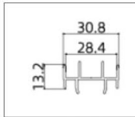
AB8010 (End Cap)
