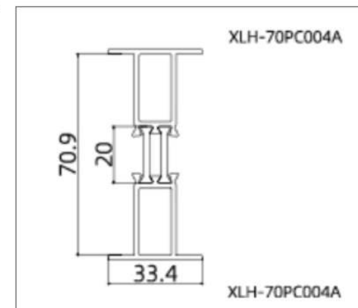
XLH-70PC004 (Mullion Bar)
