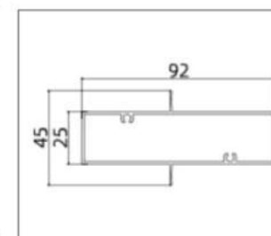
AB8018 (Frame)
