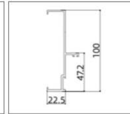
TC119003 (Side Frame)
