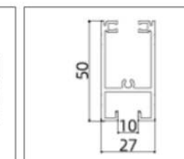
AL-9004-2.0 (Door Rail)
