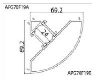
APG70F19 (90° Corner)
