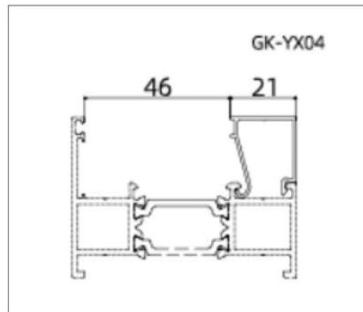
GK-YX04(Glazing Bead)
