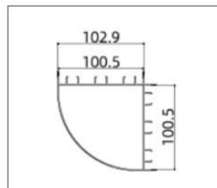
AB8022( 90° Corner)
