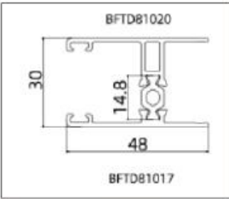
Lock Stile
