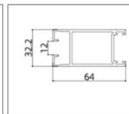
GH-TM21025 (Lock Stile)
