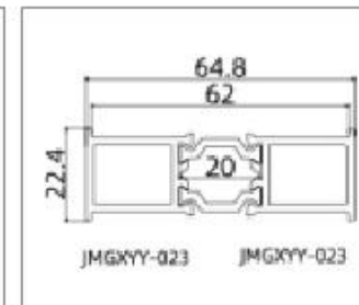
JMGXXY-GPM60108 (Mullion Bar)
