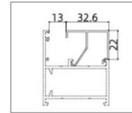
XD-5004JH-25-23C (Glazing Beadr)
