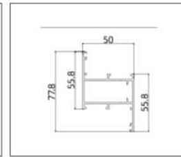
XD-5008 (Mullion)
