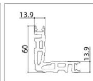
MD13.9 (Corner Connector)
