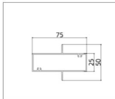
AB8006A (Transom)
