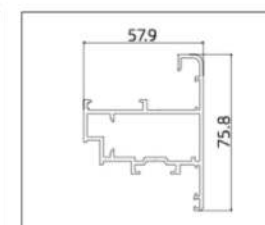
XD-5009NJH-23C (Corner Connector)
