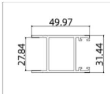
XLH-85TC010 ( Lock Stile)
