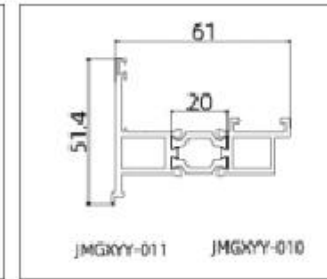
JMGXXY-GPM60104 (Frame)
