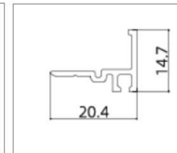
Jamb(Tooling Pending)
