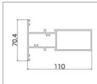
AL-PKC5002B (Mullion)
