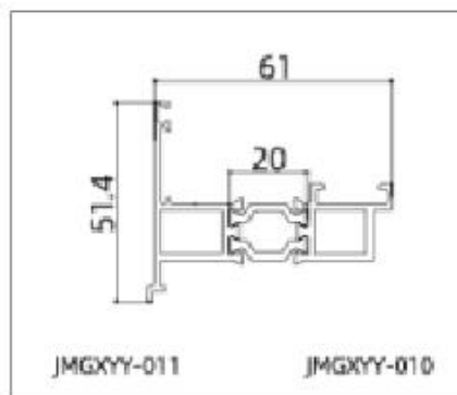
JMGXYY-GPC60104 (Frame)
