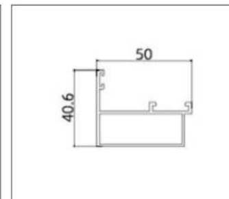
AL-PKC5011 (Frame)
