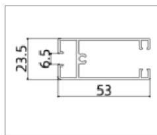
AB8014 (Door Rail)
