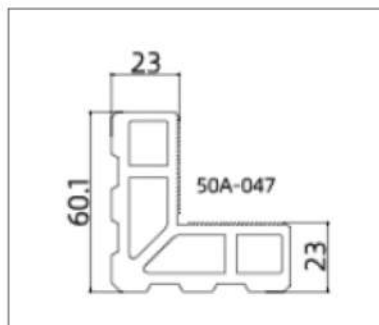
50A-047 (Corner Connector)
