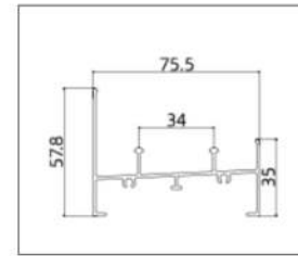
AB8003-1.35A (Track)
