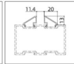
AL-9022(Glazing Bead)
