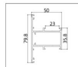
XD-5003JH-23C (Mullion)
