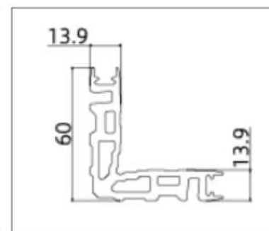
MD13.9 (Corner Connector)
