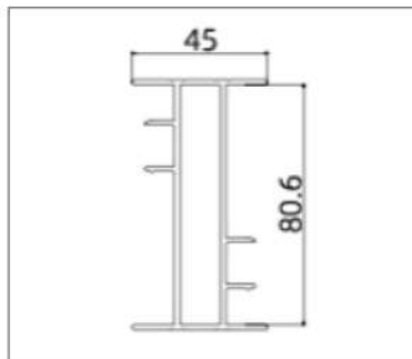
XLH-85TC011 ( Side Frame)
