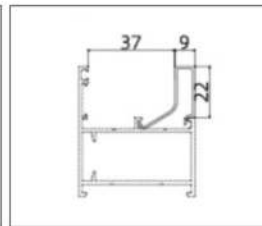
XD-5010 (Glazing Beadr)
