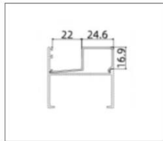
BG-PC50120 (Glazing Bead 22)
