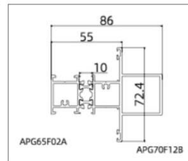
APG55F012(Mullion)
