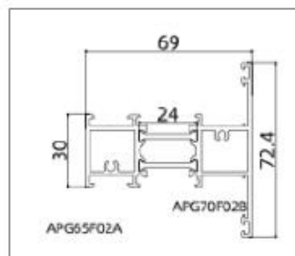
APG70F02 (Mullion)
