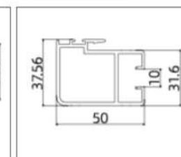
AL-9007-2.0 (Striker Stile)
