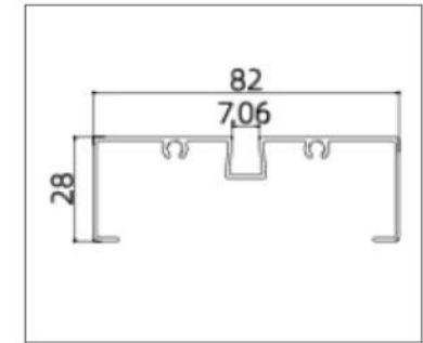
GH-85T19 (Frame)
