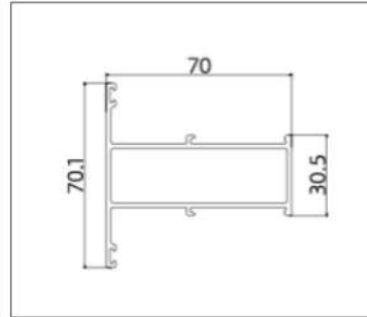
ALP7002 (Mullion)
