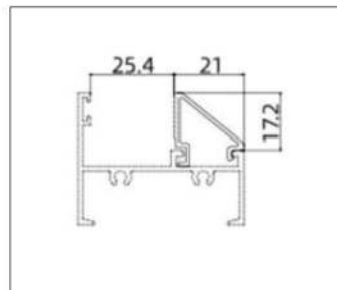
AL-PKC5004 (Glazing Bead 25.4)
