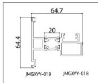
JMGXXY-GPM65106 (Mullion)
