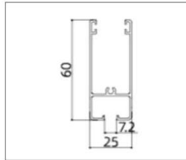
AK8205 (Door Rail)
