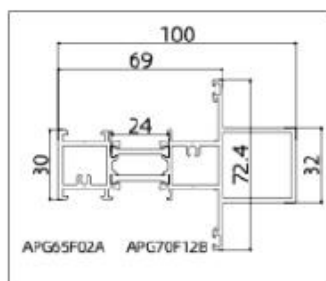
APG70F12 (Mullion)
