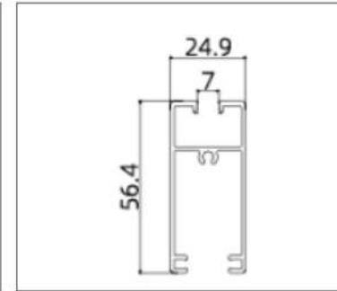
A8209 (Door Rail)
