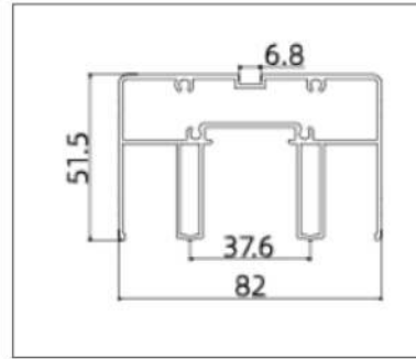
AK8201A (Top Track)
