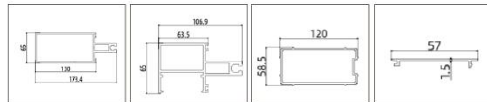
KQS13001(Mullion) Thickness:3.0mm Weight: 4.125kg/m KQS13002( ) Thickness:2.5mm Weight: 2.702kg/m KQS13003(reinforcing core) Thickness: 2.2mm Weight: 2.06kg/m YLH06BC(Frame Cover) Thickness:1.5mm Weight: 0.268kg/m
