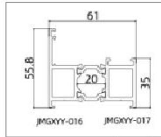
JMGXXY-GPM60101 (Frame)
