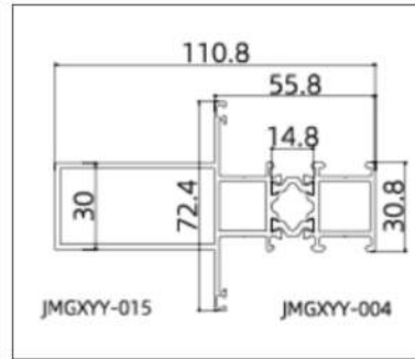
JMGXYY-GPC55112 (Mullion)
