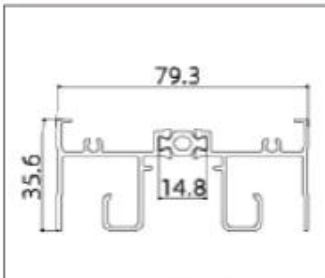
BFTD81001 (Track)
