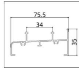
AB8003-11.5 (Track)
