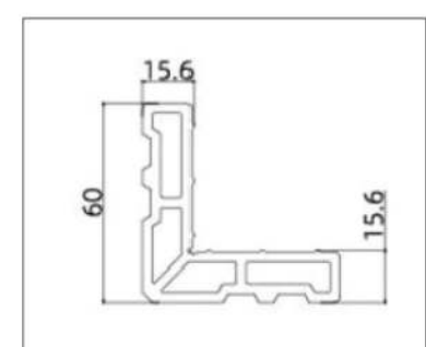
AL-PKC5013(Corner Connector)
