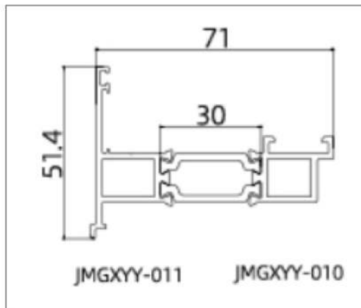
JMGXYY-GPC70104 (Frame)
