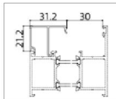
APG70F030 (Glazing Bead)
