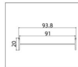
AL-9016 (Mullion Bar)
