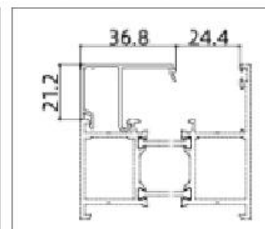
APG70F010 (Glazing Bead)
