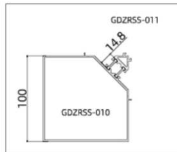
JMGXYY-GPM55109(90° Corner)
