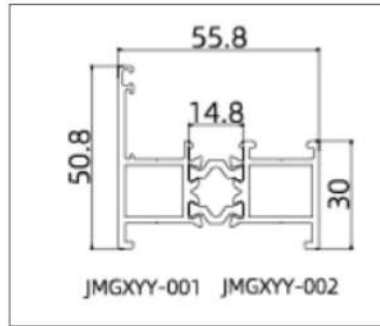
JMGXYY-GPC55101 (Frame)
