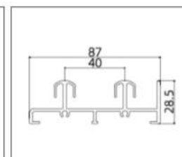
AL-9002-2.0 (Track)
