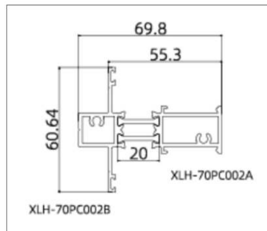
XLH-70PC002 (Mullion)
