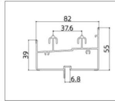
AK8202 (Roller Track)
