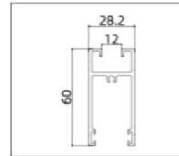
TC119008 (End Cap)
