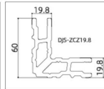
DJS-ZCZ19.8(Frame)
