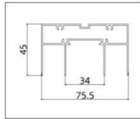
AB8002-0.95 ( Track )
