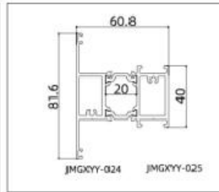
JMGXXY-GPM60102 (Mullion)
