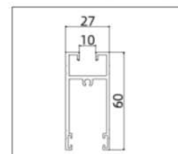
AL-9005-2.0 (Door Rail)
