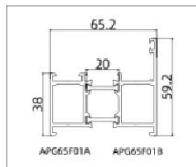
APG65F01 (Frame)
