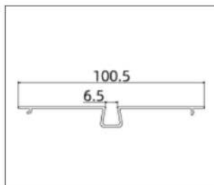
AB8021 (Interlock)
