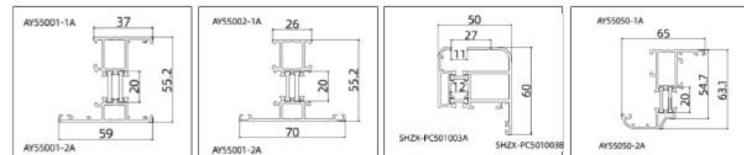
AYPD55001 (Frame)
