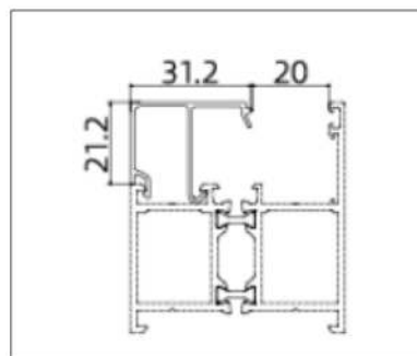
SHZX-PC501020 (Glazing Bead)
