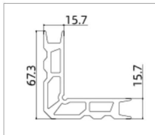
BFUS20922(Corner Connector)
