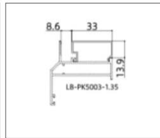
LB-PK5030 (Glazing Bead 8.6)
