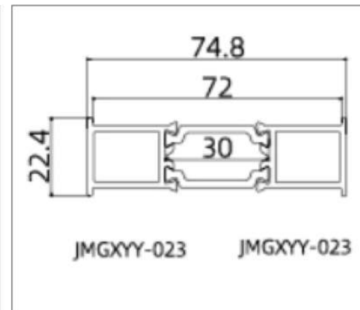
JMGXYY-GPC70108 ( Mullion Bar )
