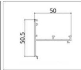
XD-5011 (Frame)
