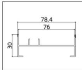
AB8004-11.5 (Frame)
