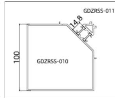
JMGXYY-GPC55109 (90° Corner)
