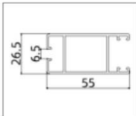
AB8013-1.15 (Lock Stile)
