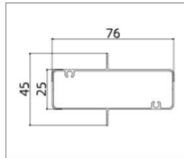
GH-85T09 (Mullion)
