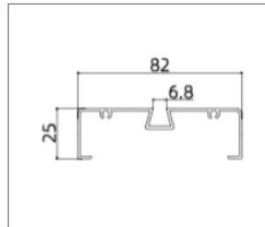
AK8209 (Frame)
