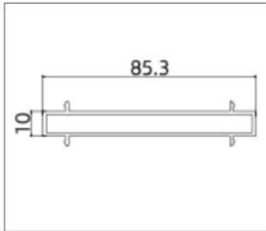
AK8212 (Mullion Bar)
