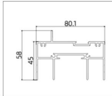
XLH-85TC006 (Track)
