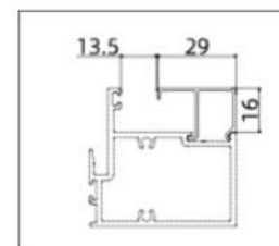
GH-TM21007 (Glazing Bead)
