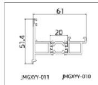
JMGXXY-GPM65104 (Frame)
