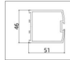
AL-DTM4601(460 Transom)
