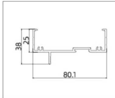
XLH-85TC005 (Frame)
