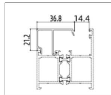
APG55F010 (Glazing Bead)
