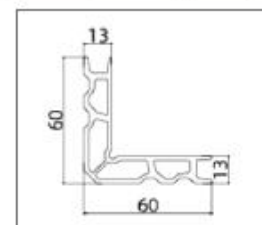
BFUS20915 (Corner Connector)
