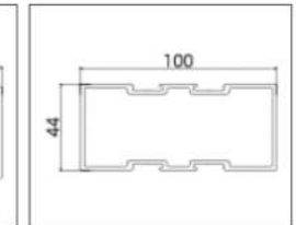
GH-GD002 (Mullion Bar)
