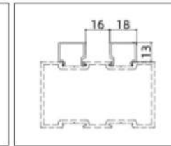
BFTB08051(Glazing Bead)
