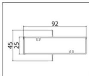
AB8020 ( Frame Cover)
