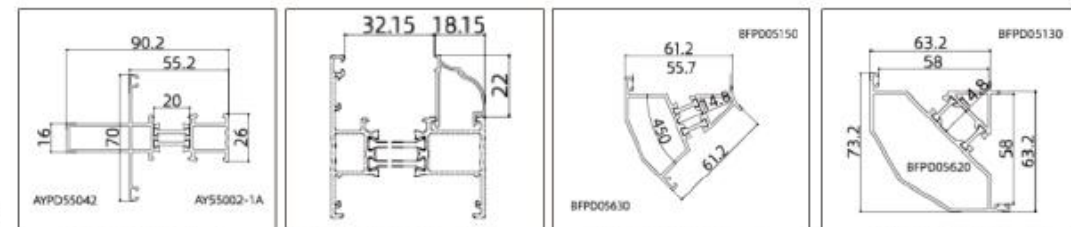
AYPD55004 (Mullion)
