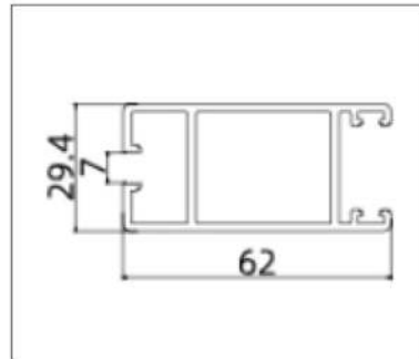
A8210-1.8 ( Lock Stile)
