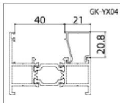
GK-YX04 (Glazing Bead)
