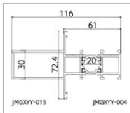
JMGXYY-GPC60112 (Mullion)
