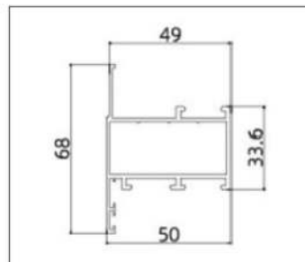
AL-PKC5003 (vent)
