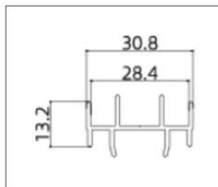
AB8010 ( End Cap)
