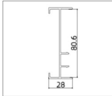
XLH-85TC001 (Side Frame)
