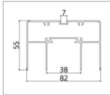
GH-85T01 (Track)
