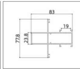
XD-5003JQ-83 (Mullion)
