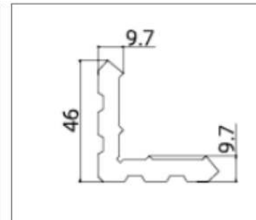
AL-PKC5014( Frame)
