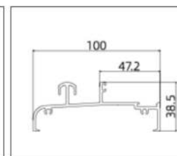
GH-TM21003 (Track)
