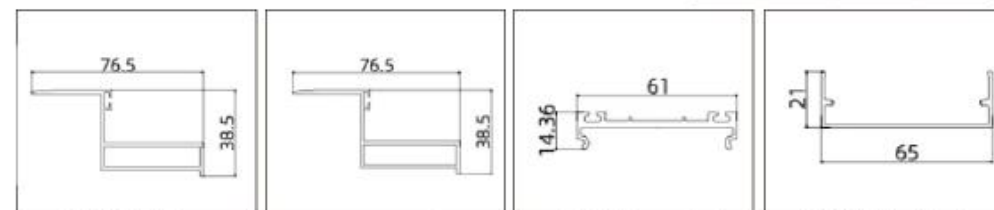
KQS13050(Sash) Thickness:1.5mm Weight: 0.721kg/m KQS13051(Sash) Thickness:1.5mm Weight:0.721kg/m KQS15007(pressure plate) Thickness: 2.6mm Weight: 0.642kg/m KQS15008(Frame Cover) Thickness:1.2mm Weight: 0.382kg/m
