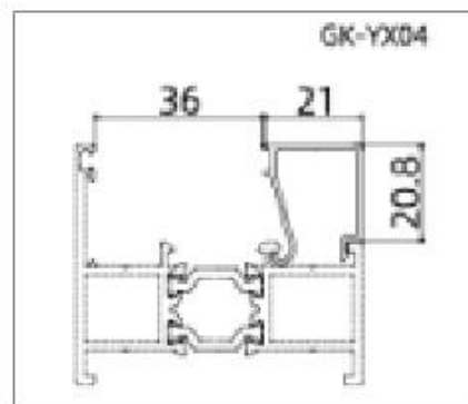
50A-047 (Corner Connector)
