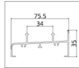
AB8003-1.35A (Track)
