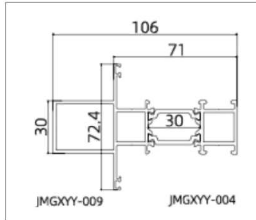
JMGXYY-GPC70102 (Mullion)
