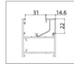
XD-5004JH (Glazing Beadr)
