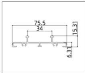
AB8026-1.2 (Track)
