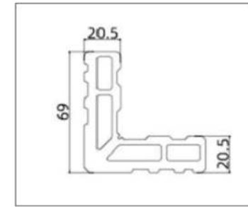
AL-PKC5012 (Corner Connector)
