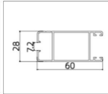
AK8206 (Lock Stile)
