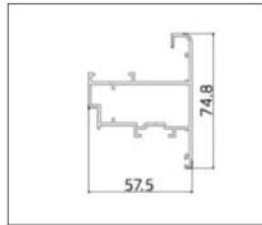
XD-5009N2 (Vent)
