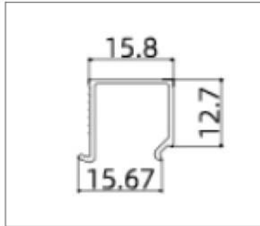
XLH-85TC003 (Glazing Bead)
