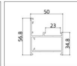
XD-5001JH-23C (Glazing Beadr)
