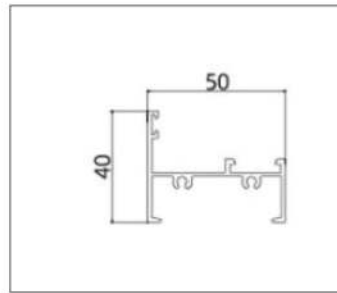
AL-PKC5001 (Frame)
