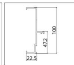
GH-TM21004 (Side Frame)
