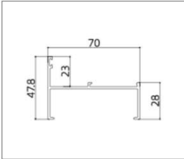
ALP7001 (Frame)
