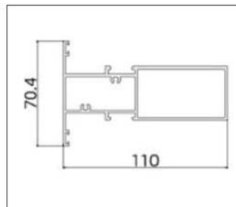
AL-PKC5010 (Frame)
