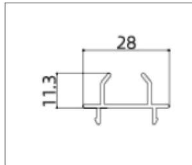
AK8208 (End Cap)
