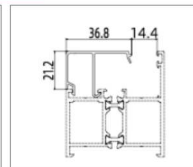
APG60F010 (Glazing Bead)
