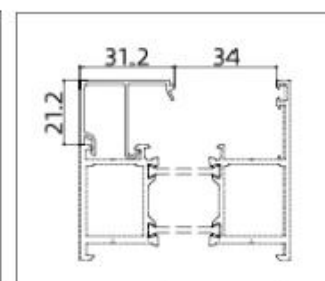
APG70F30 (Glazing Bead)
