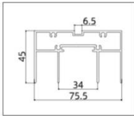
AB8002-1.35 (Track)
