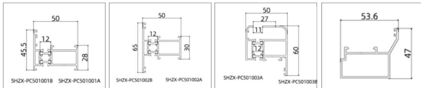
SHZX-PC501001 (Frame)
