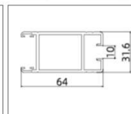
AL-9006-2.0 (Lock Stile)
