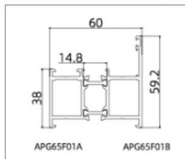
APG60F01 (Frame)
