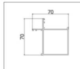
XD-5009NJH-23C (Glazing Beadr)
