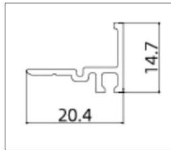
Jamb(Tooling Pending)
