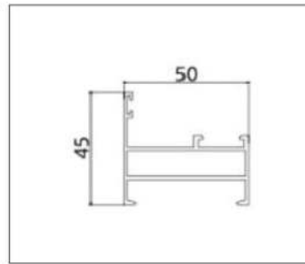
AL-PKC5001A (Frame)
