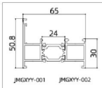
JMGXYY-GPC65101 (Frame )
