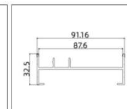
AL-9003-2.0 (Frame)
