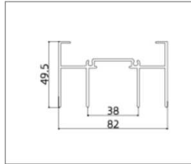
A8202 (Track)
