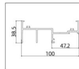
GH-TM21001 (Track)
