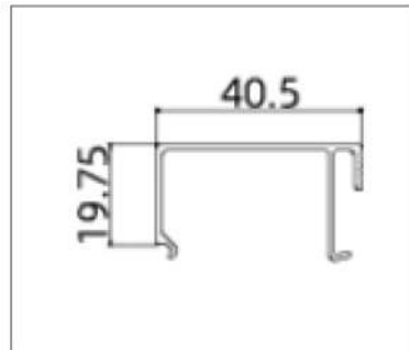
ALP7005 (Glazing Bead)
