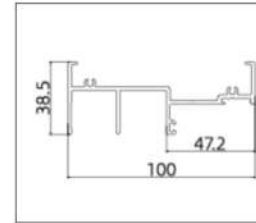
TC119001 (Track)
