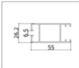
AB8013-0.95 (Lock Stile)
