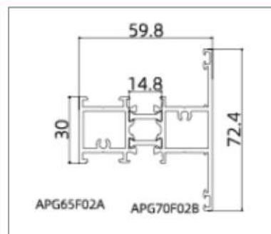
APG60F02 (Mullion)
