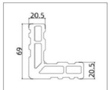
AL-PKC5014 (Corner Connector)
