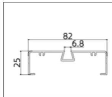
AK8209 (Frame)
