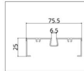
AB8007-0.95 (Frame)
