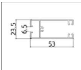
AB8014 (Door Rail)
