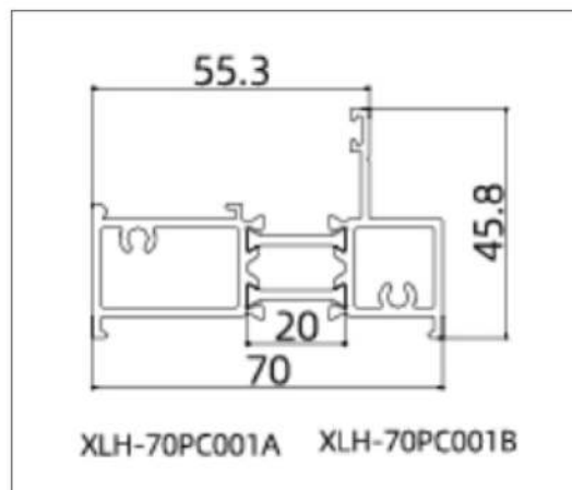
XLH-70PC001 (Frame)
