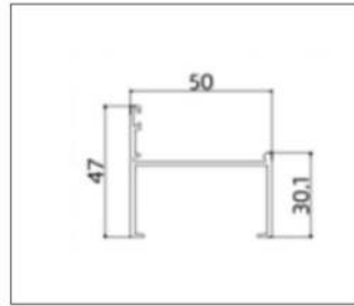
LB-PK5001-1.35 (Frame)
