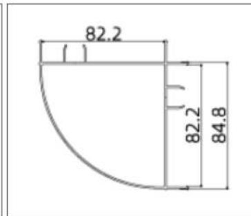
GH-85T13 (90° Corner)
