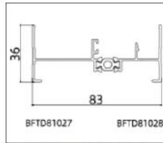
BFTD81022 (Glazing Bead)
