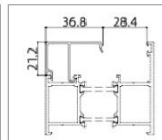
APG70F010 (Glazing Bead)
