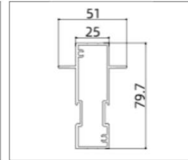
XLH-85TC004 (Mullion)
