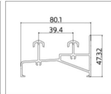
XLH-85TC009 (Door Rail)
