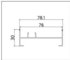
AB8004-0.95 (Frame)
