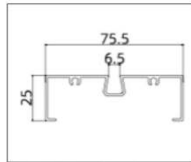
AB8007-1.15A ( Frame)
