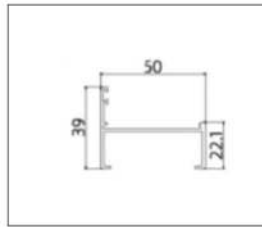
XD-5003G (Mullion)
