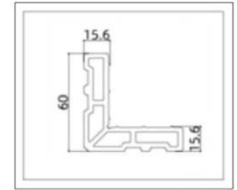
BG-PC50103 (Corner Connector)
