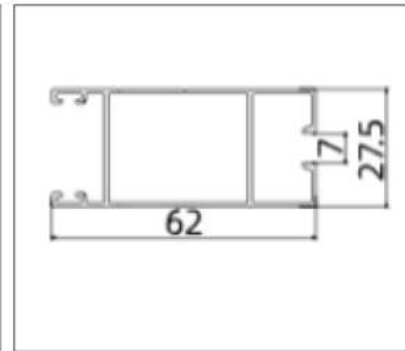
GH-85T06 (Lock Stile)
