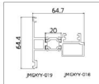
JMGXXY-GPM60106 (Mullion)
