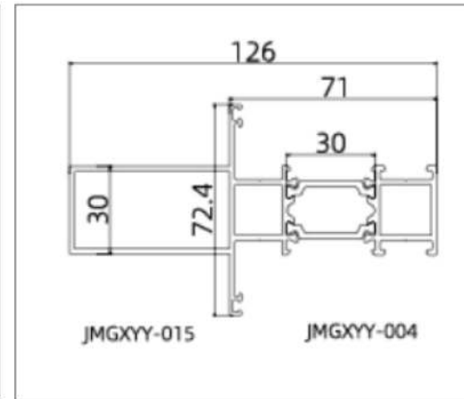
JMGXYY-GPC70112 (Mullion)
