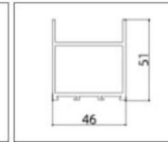
AL-DTM4603(460 Transom)
