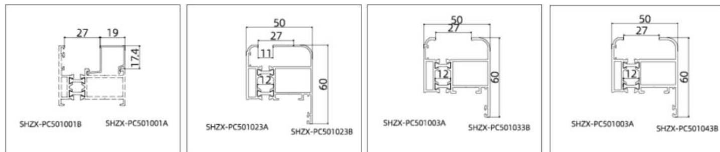
SHZX-PC501020 (Glazing Bead)
