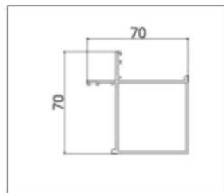
LB-PK5008(90° Corner)
