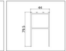
AL-DTM4604(460 Transom)
