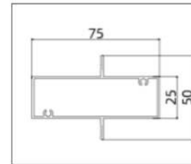
AB8006A (Transom)
