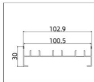
AB8017 (Side Frame)
