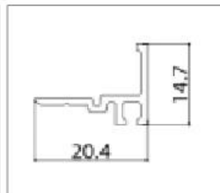
Guide Rail (Mold Pending)
