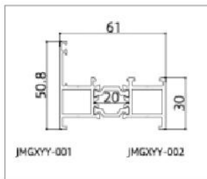
JMGXYY-GPC60101 (Frame)
