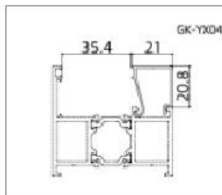
GK-YX04 (Glazing Bead)
