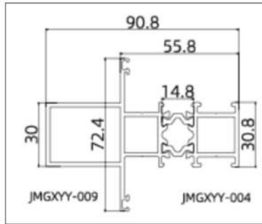
JMGXYY-GPC55102 (Mullion)
