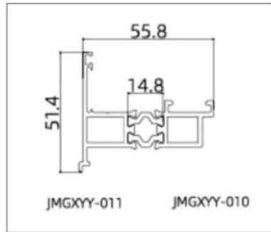
JMGXYY-GPC55104 (Frame)
