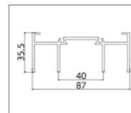
AL-9001-2.0 (Track)
