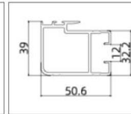
TC119010 (Track)
