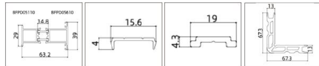
BFPD05540(Mullion Bar)
