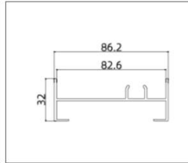
A8204-1.8 (Frame)
