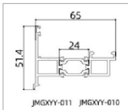
JMGXYY-GPC60104 (Frame )
