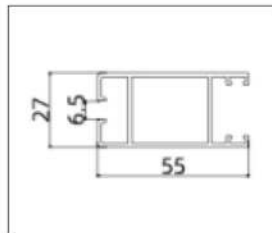
AB8013-1.35A (Lock Stile)
