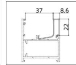
XD-5010JH-23C (Glazing Beadr)
