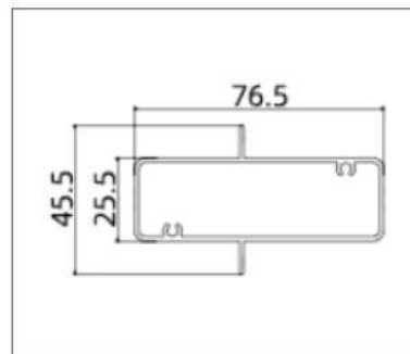
AK8210 (Transom)
