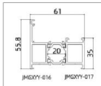
JMGXXY-GPM65101 (Frame)
