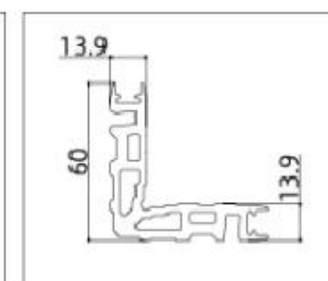
MD 13.9 (Glazing Bead)
