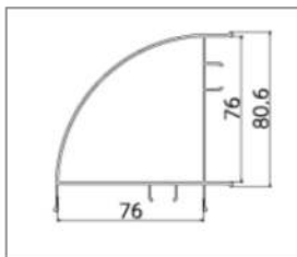
AB8011A (90° Corner)
