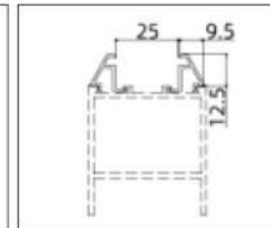
AL-DTM4606(Glazing Bead)
