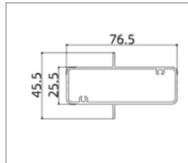
AK8210 (Transom)
