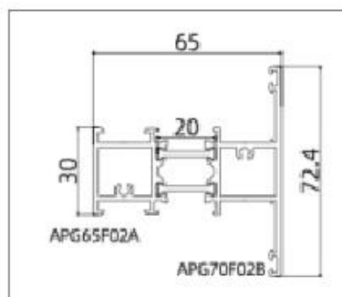
APG65F02 (Mullion)
