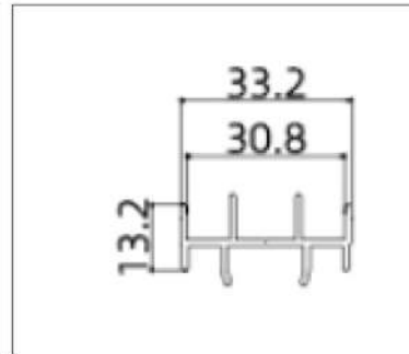
A8216 ( End Cap )
