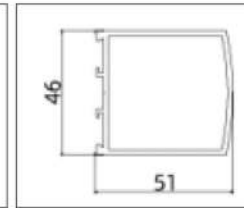
AL-DTM4602(460 Transom)
