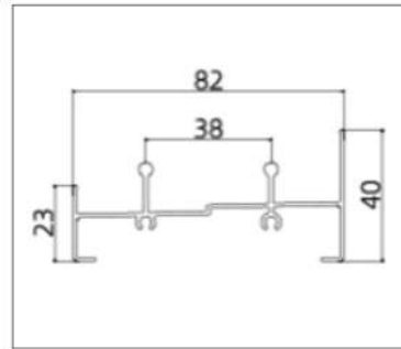
GH-85T02 (Track)
