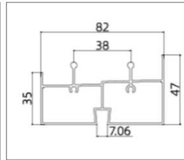
GH-85T12 (Frame)
