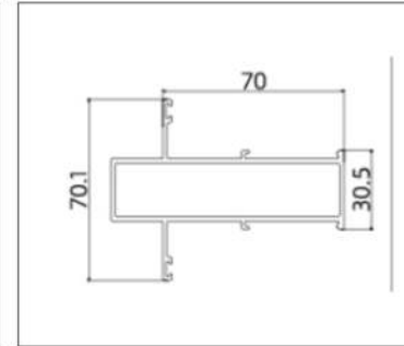
ALP7012 (Mullion)
