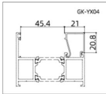
GK-XY04 (Glazing Bead)
