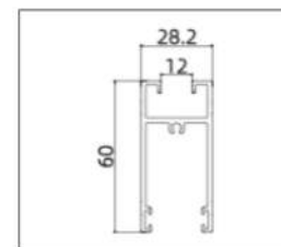
GH-TM21015 (Door Rail)
