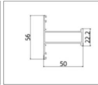
LB-PK5002-1.35 (Mullion)
